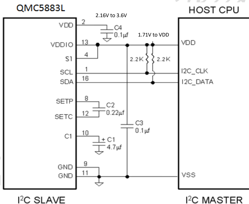
Figure 5. Dual Supply Connection
