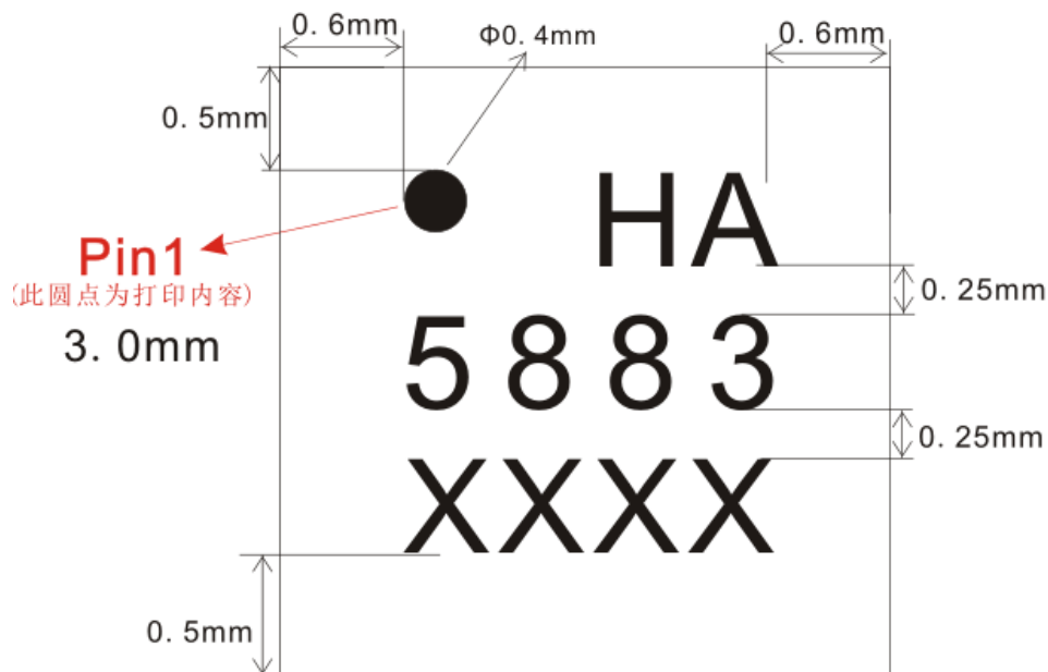
Figure 4. Chip Marking
