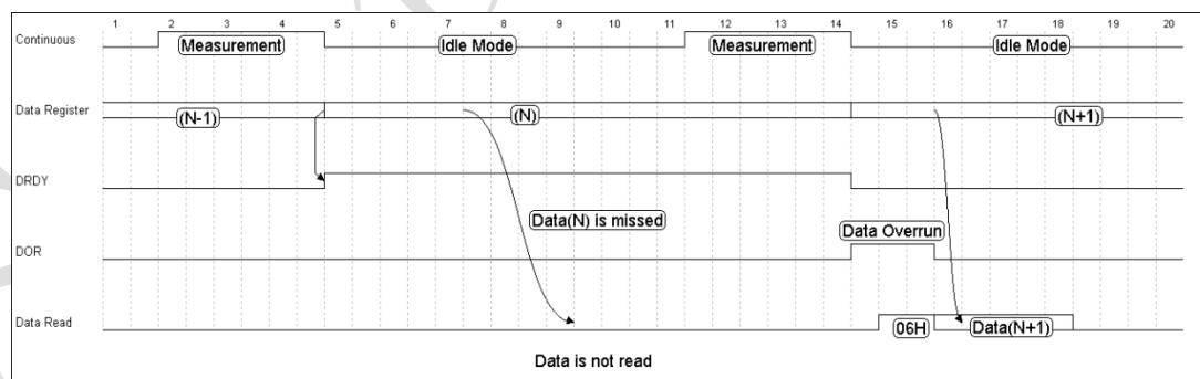
Figure 12. Sequence When Data Not Read
