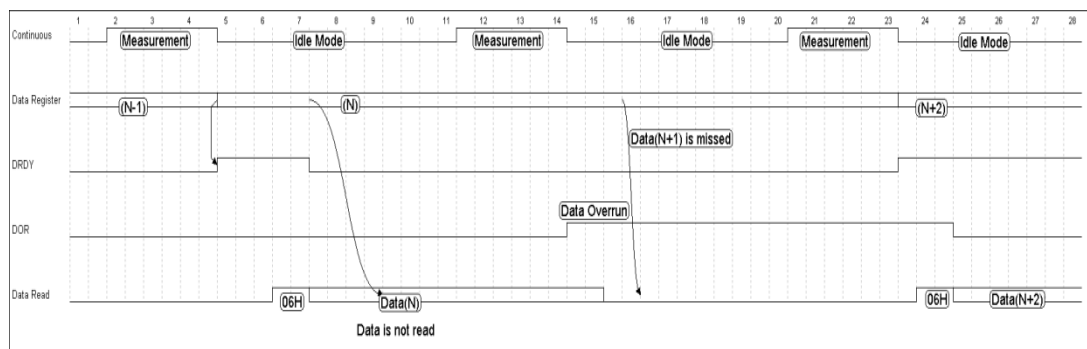
Figure 13. Sequence When Data Locks
