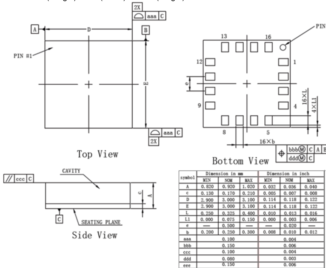
Figure 3. Package Size
