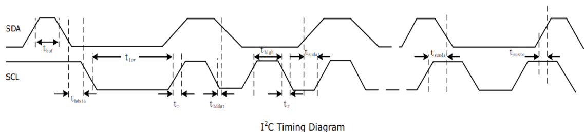
Figure 14. I 2 C Timing Diagram
