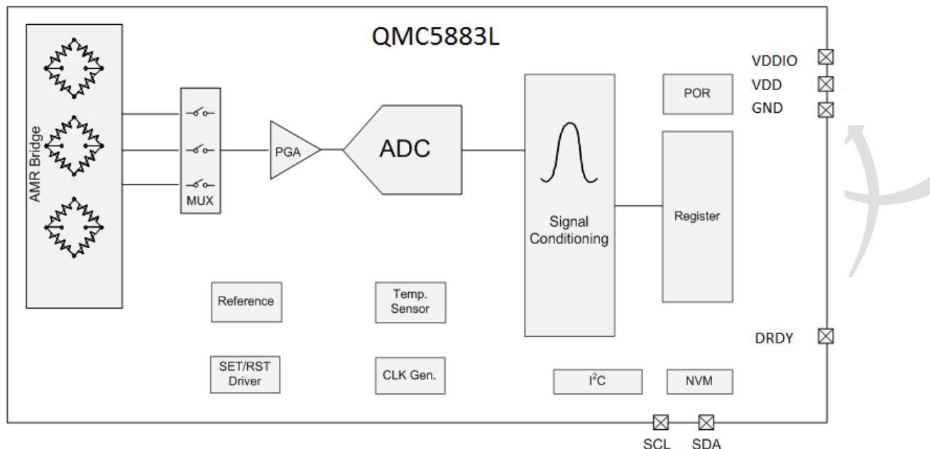
Figure 1. Block Diagram
